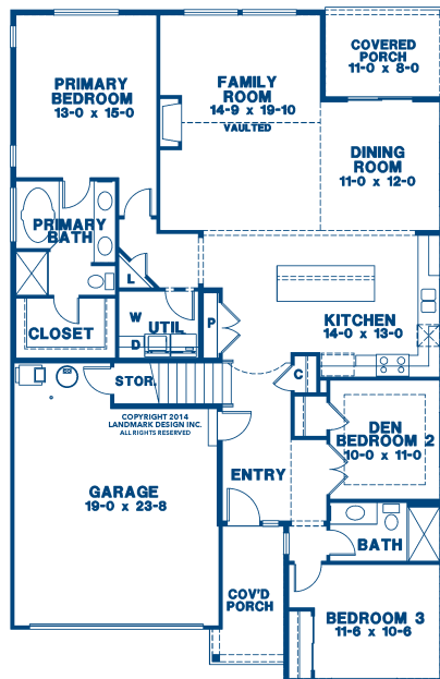
MAIN FLOOR PLAN
